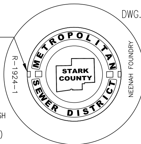
NEENAH LOGO LID: NF-19245004
