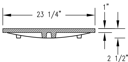
EJ LOGO LID: 1850A PRODUCT # 00185032
